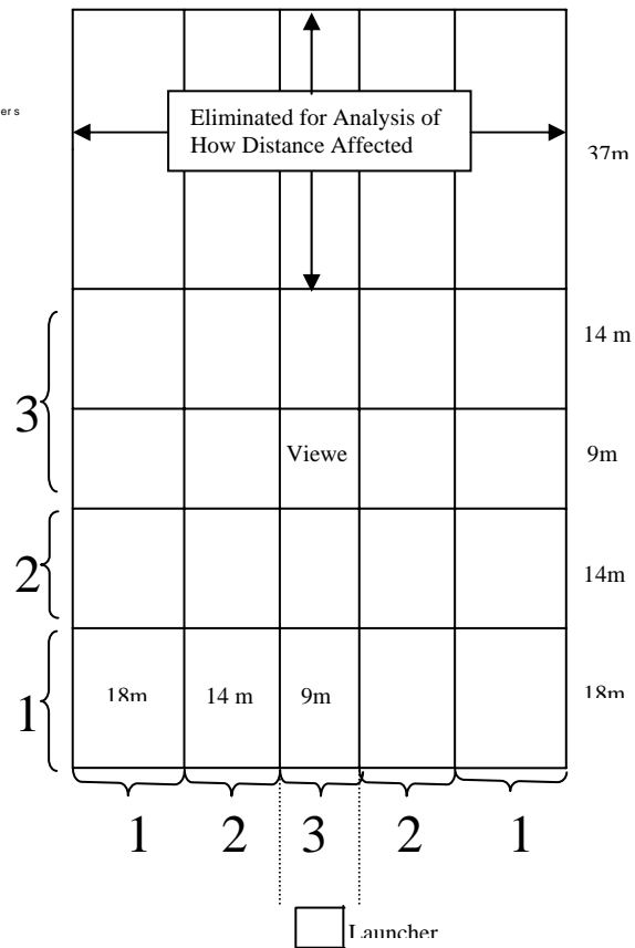
Figure 7. Categorization of distances from observers for analysis. This figure shows the general layout of the field from figure 5. The numbers listed along the rows and columns indicate how distance was categorized in the lateral and depth direction for the analysis of landing distance and apex estimation.
