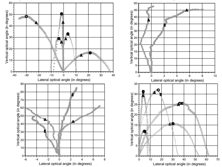
Figure 5. Optical ball trajectories in the treatment condition. (top left panel) Shown are empirical optical trajectories and the exact frame in time of the actual apex (‘A’), participants’ mean estimate (‘E’) and the optical apex (‘O’) occurs for balls landing in front of participants. Each frame represents the optical position of the ball (relative to where the observers are looking) at each 1/30 th of a second video frame. (top right panel) Shown are the empirical optical trajectories for balls landing very close to participants. In the trajectory on the left, only the actual apex (A) is shown because participants’ indications and the optical apex occur long after the portion of the optical trajectory shown. (bottom left panel) Shown are the empirical optical trajectories for balls going over the heads of participants. Shown also is exactly what frame in time the Actual apex occurs. In all the trajectories only the actual apex (A) is shown because estimations and the optical apex occur long after the portion of the optical trajectory shown. (bottom right panel) Shown are the empirical optical trajectories for balls in the control conditions. The three symbols representing the actual apex (‘A’), the optical apex (‘O’) and participants’ estimations (‘E’) are shown.
