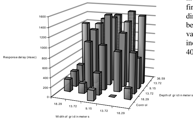
Figure 6. Delay between participant’s estimations of when the apex occurred and when it actually occurred. Shown is the response delay in milliseconds (msec) between participants’ responses and the physical apex for ball trajectories landing in the respective grids. The bar at the very front represents the delay for the control conditions.
