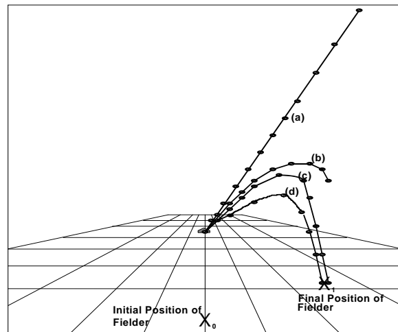
Figure 3. Questionnaire given to participants concerning what the trajectory of a fly ball looks like from the perspective of a fielder fielding the ball. Participants were asked to indicate what the trajectory looks like from the perspective of a fielder running to make the catch. Trajectory (a) is what the veridical optical trajectory from the perspective of the fielder
