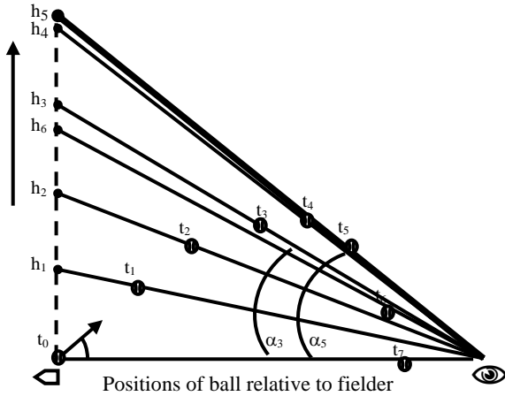
Figure 2. The occurrence of the physical and optical apices for a stationary fielder toward whom the ball is launched. In these cases, the optical apex occurs much later than the physical apex. Physical points in time of the ball ( t ) are shown along with optical points in time ( h ) that correspond to the physical points.
