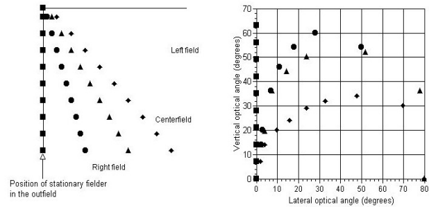
Figure 1. Bird's-eye view of four ball trajectories relative to a stationary fielder. (left panel) Bird's eye view of four ball trajectories starting at the same position and landing in different positions on the field is shown (ignoring effects of air resistance and ball spin). (right panel) Optical ball trajectories of a stationary fielder for the four trajectories shown in the left panel of figure 1. The perspective optical parabolas appear narrower and their apparent apices are later as the destination point physically approaches the fielder.
